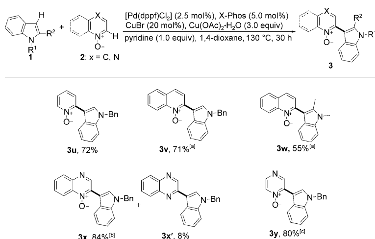
Scheme 4. Selective oxidative cross-coupling of indoles with a variety of N-heteroarene N-oxides. For all reactions 0.5 mmol indole 1 and 3.0 equiv N-heteroarene N-oxide 2 were used under an N 2 atmosphere. Yields of isolated product is based on indole 1 . [a] Carried out at 110 °C, 2 (0.5 mmol), and indole 1 . [b] Pyridine (2 equiv), carried out at 140 °C.
